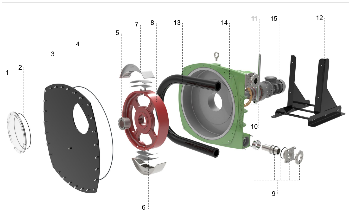
Figure 1 Layout VF 100 (Generic View)
