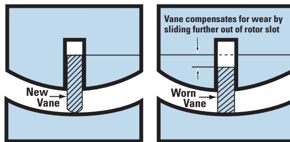
How Blackmer's sliding vanes self-adjust for wear
