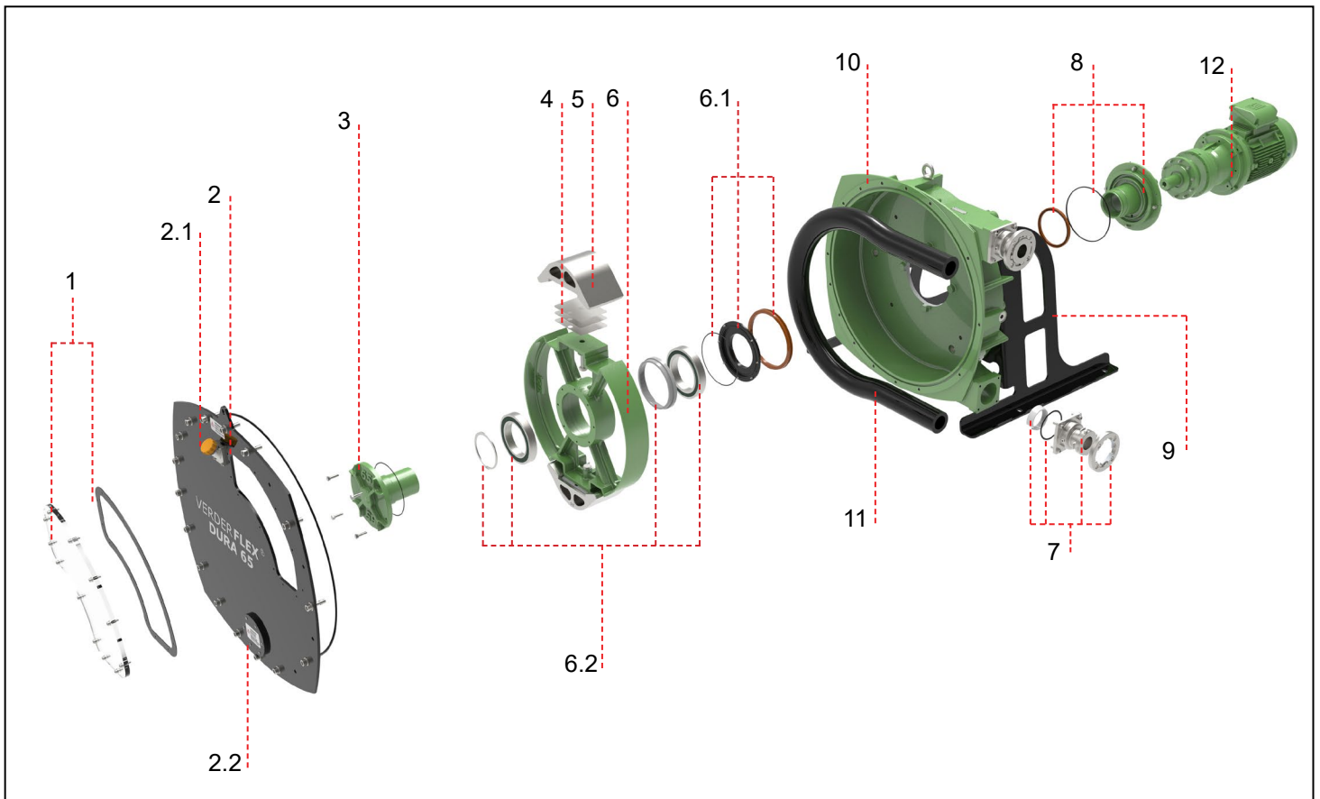
Figure 1 Layout Dura 65 (Generic View)
